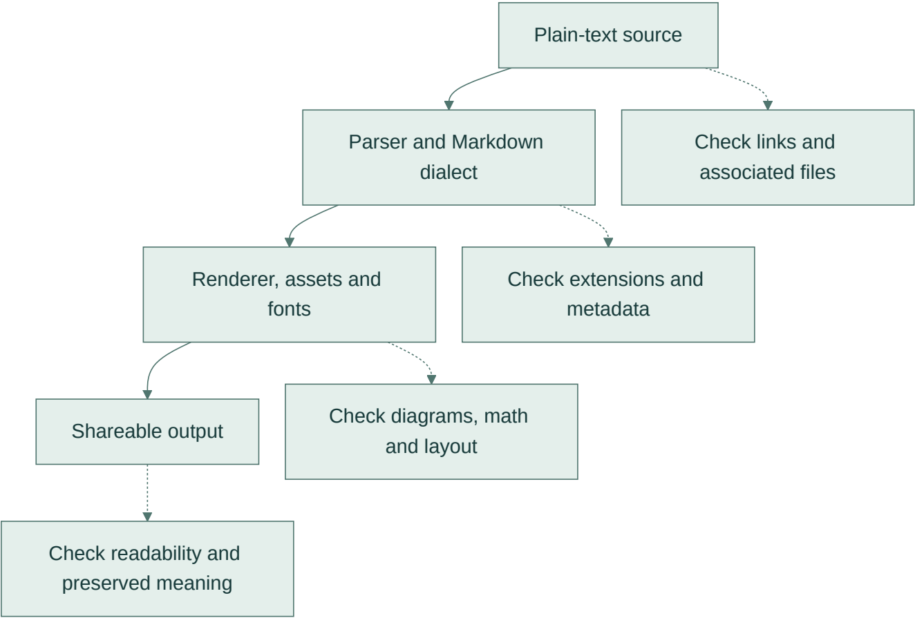
Conceptual path from Markdown source through dialect, assets and rendering to a shareable document.
